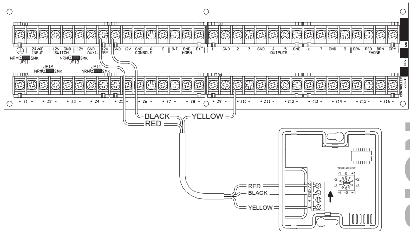
FIGURE 1 – MODEL 31A00-7 CONNECTIONS
