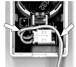
Fig. 5. Curl plug wires inside case to avoid pinching wires
