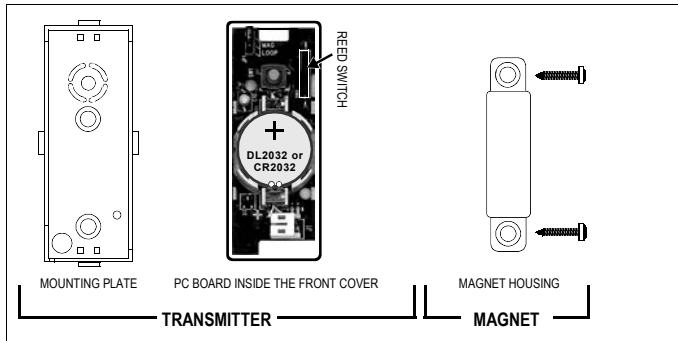
Fig. 1. GEM-TRANSLP Component Parts
