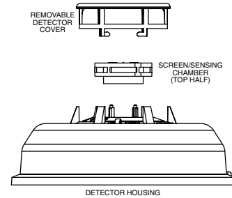
Figure 5: Removing Screen/Sensing Chamber
