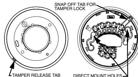
FIGURE 2: TAMPER-RESISTANT FEATURE
