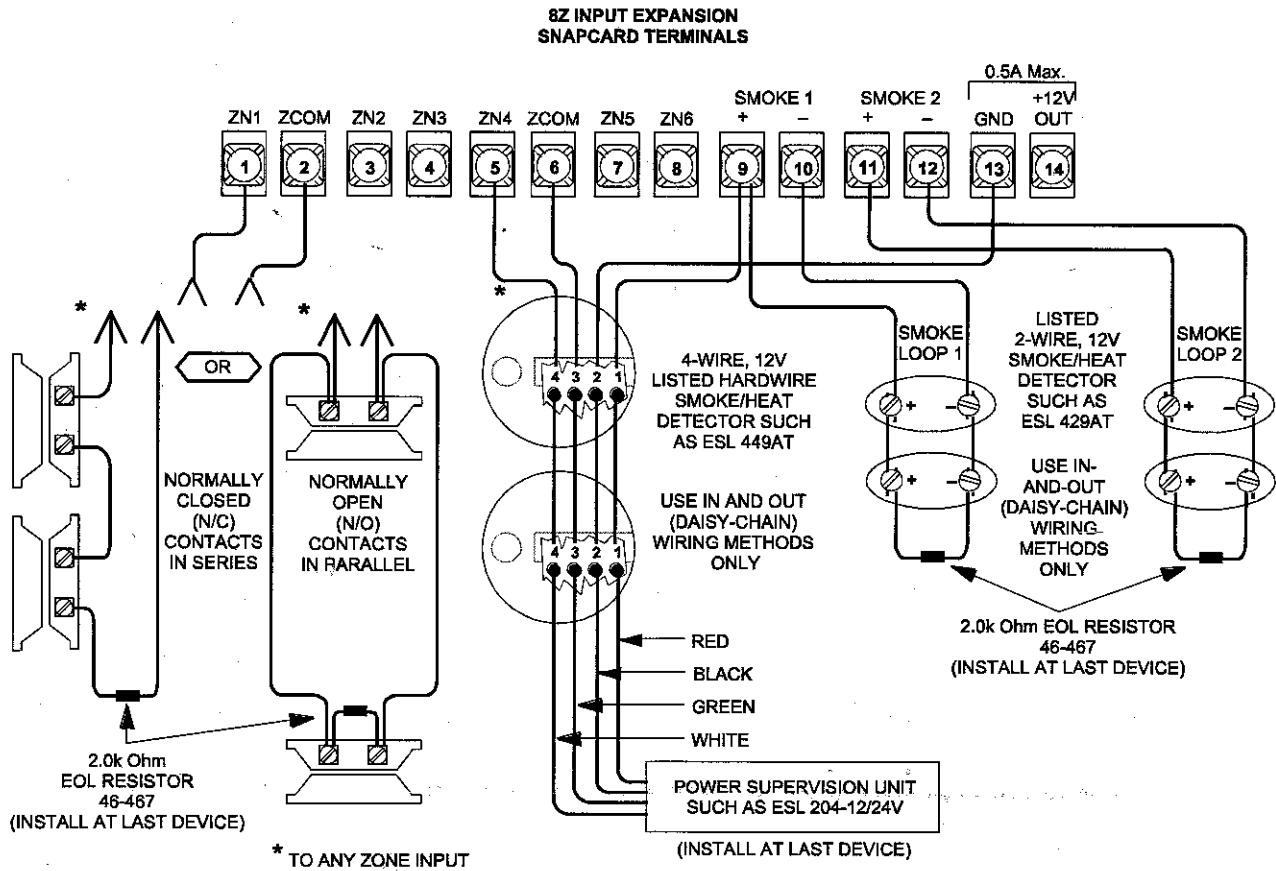
Figure 5. 8Z Input Expansion SnapCard Wiring Diagram
