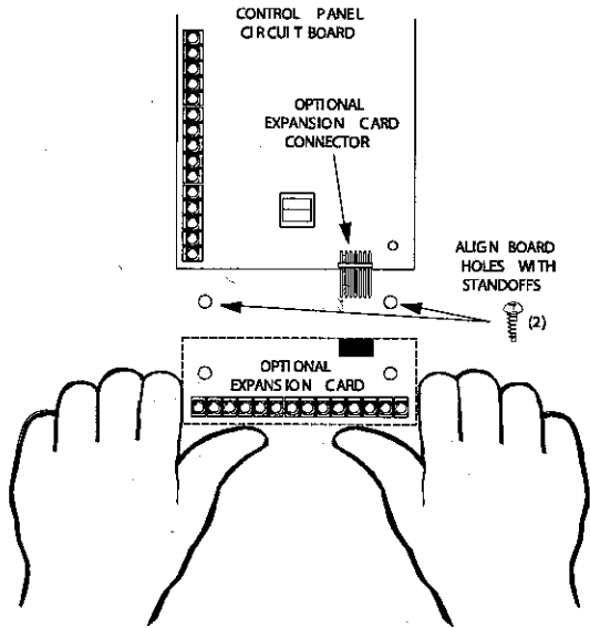
Figure 2. Concord, Concord 4, or Concord Express V4 SnapCard Installation
