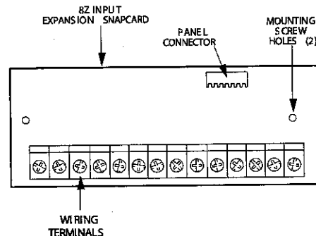
Figure 1. 8Z Input Expansion SnapCard components
