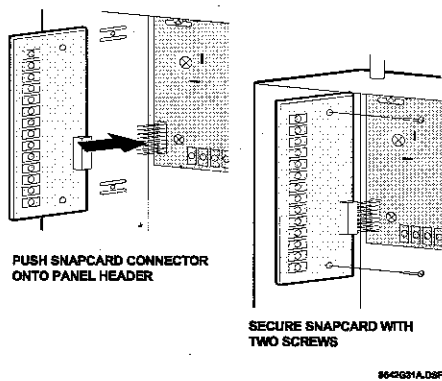
Figure 3. Concord Express SnapCard Installation
