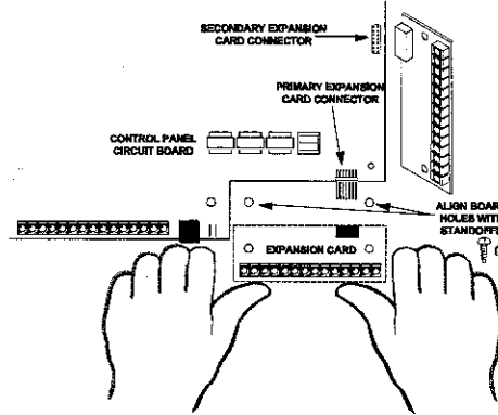
Figure 4. Advent SnapCard Installation
