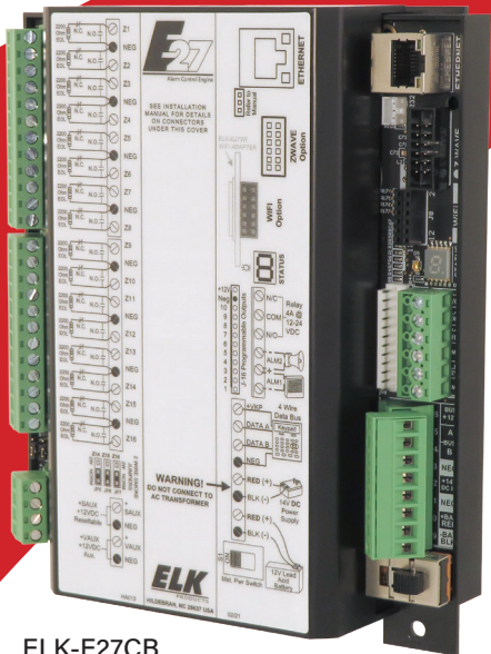
ELK-E27CB E27 Alarm Engine Control Board
